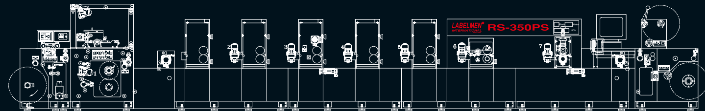
RS-350PS 5-Color Full Rotary / Intermittent Offset Printing Machine With Multi-Functional Flexo Printing Station
